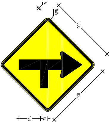
W2-4(R)(A) 600 x 600
